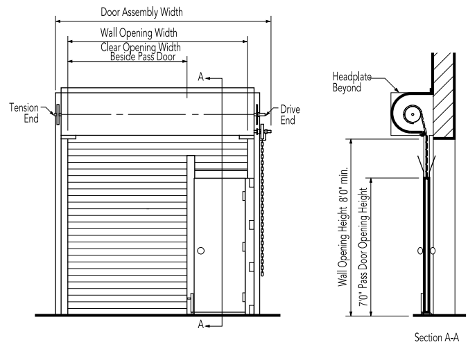
Swing-in door
